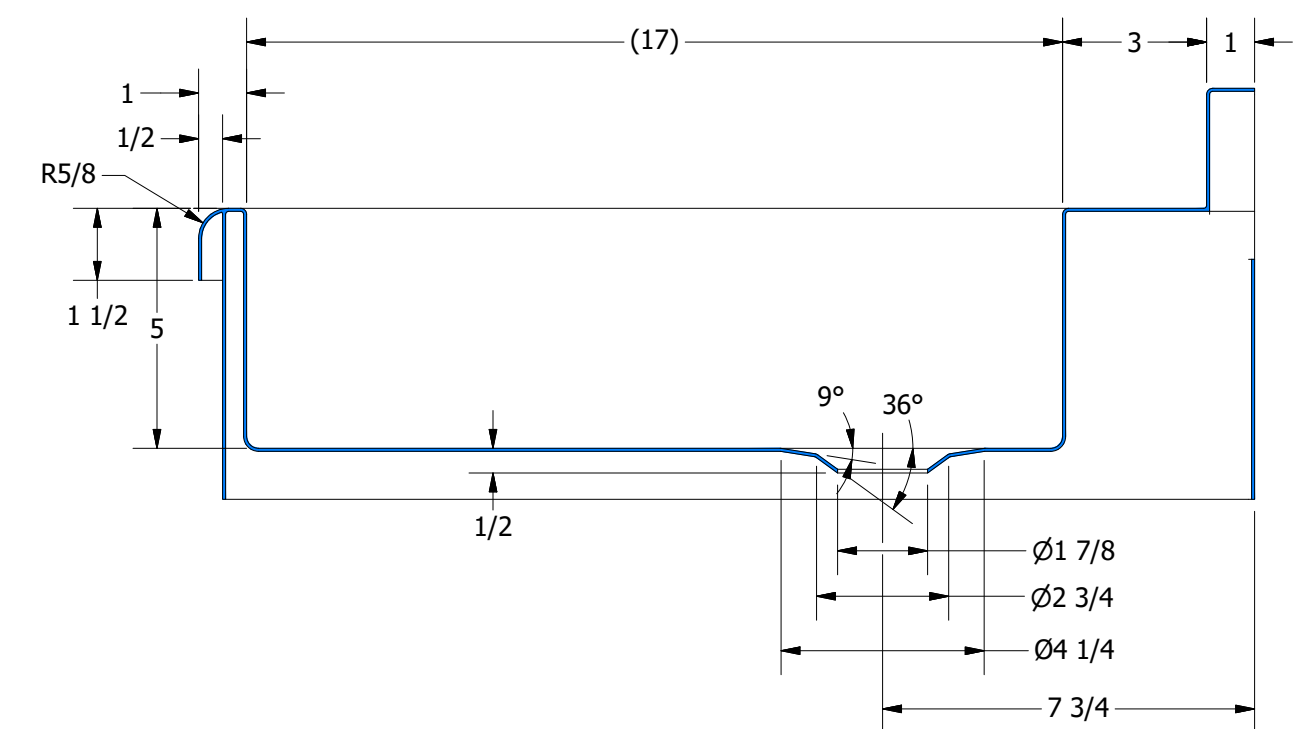
SECTION A-A SCALE 1 / 4
